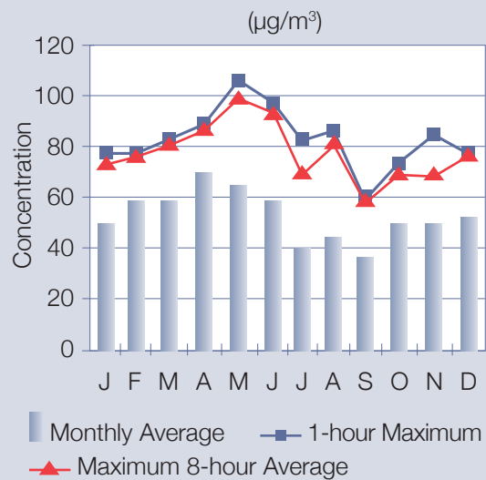
Figure 8: 2010 Yellowknife Ozone
