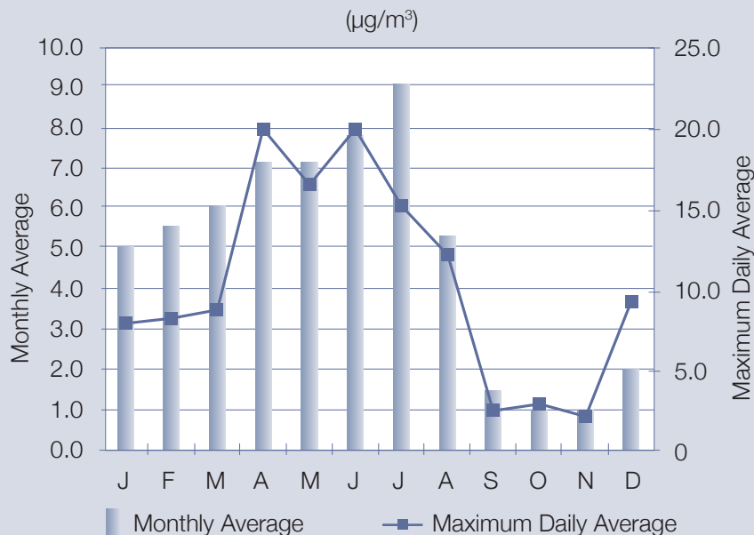
Figure 12: 2010 Inuvik BAM PM 2.5
