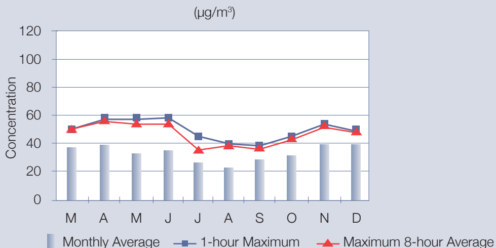
Figure 14: 2010 Inuvik Ozone
