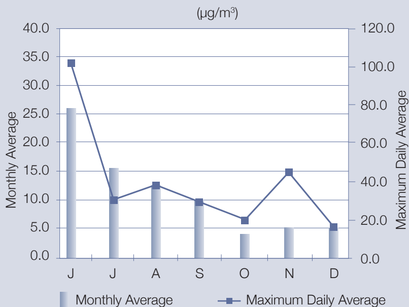
Figure 5 shows the BAM PM 10 monthly averages and maximum daily averages per month measured at the station in 2010. The highest maximum daily concentration was 100.0µg/m 3 , occurring in June.
