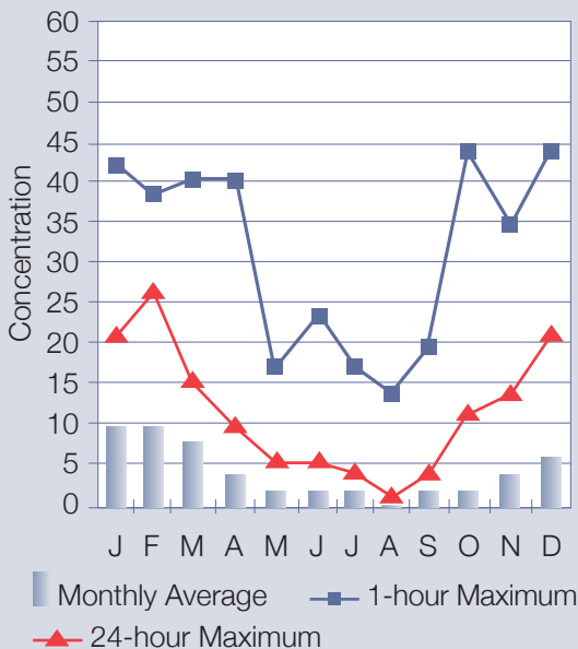
Figure 9: 2009 Yellowknife Nitrogen Dioxide (µg/m 3 )
