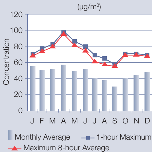
Figure 7: 2009 Yellowknife Ozone
