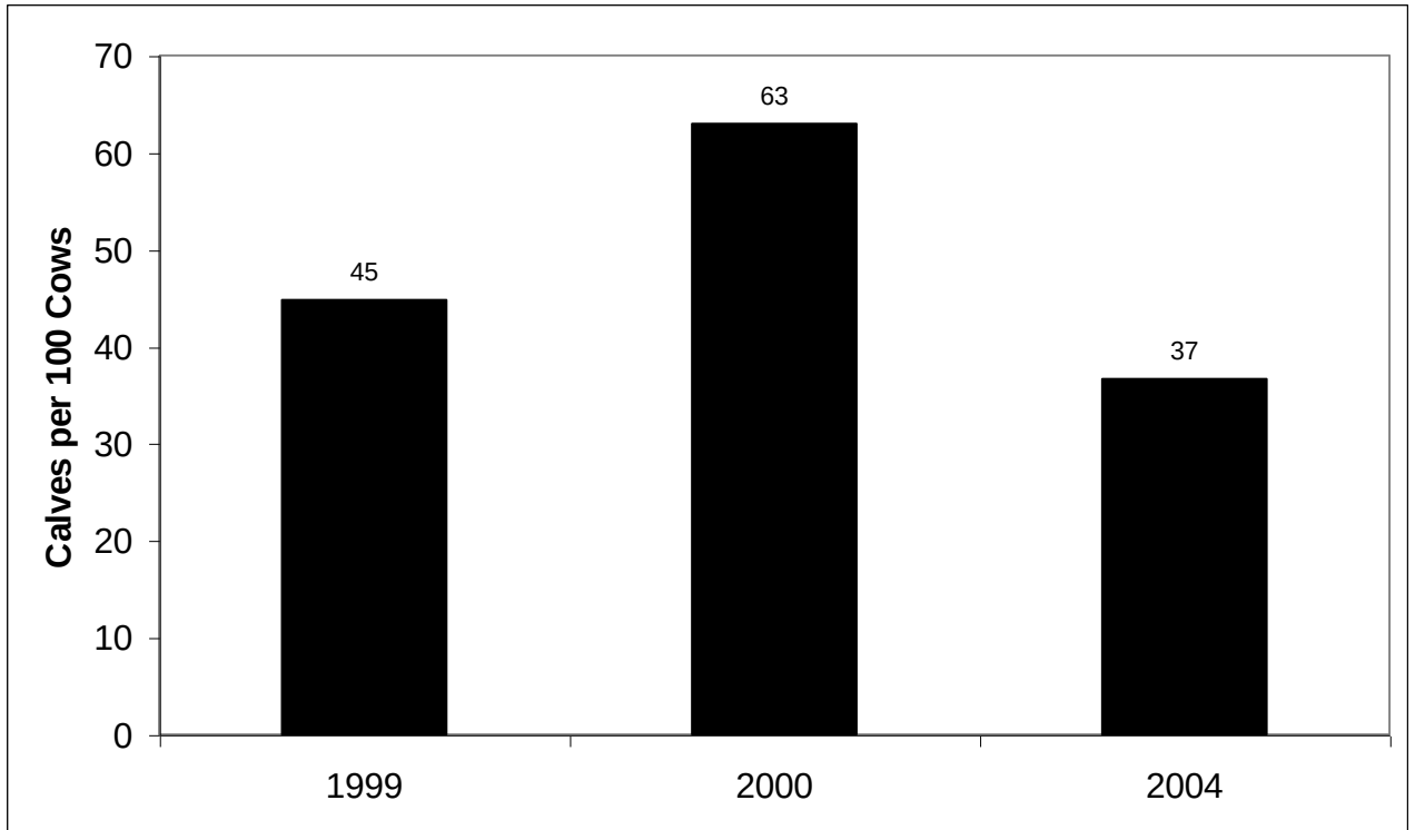
Figure 15. Calf production (number of calves per 100 adult females) for Peary caribou on Melville Island, July 1999 to 2004 A .
