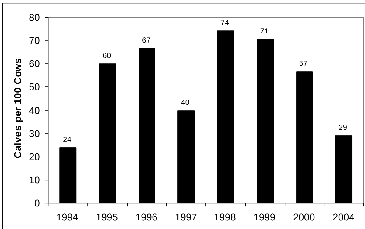
Figure 5. Calf production (number of calves per 100 adult females) for Peary caribou on Banks Island, NT, July 1994 to 2004 A .
