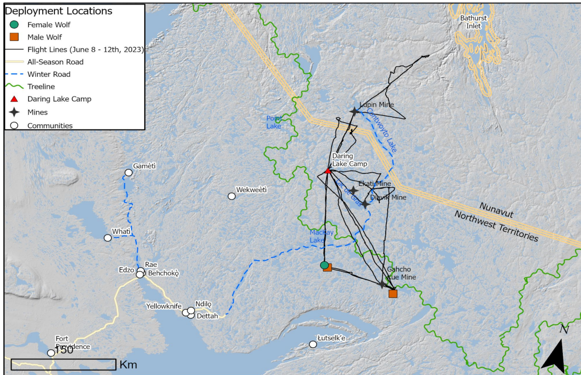
Figure 4. Flight lines and distribution of GPS/Iridium satellite collared wolves in June 2023. Efforts were based from Daring lake camp (red triangle).
