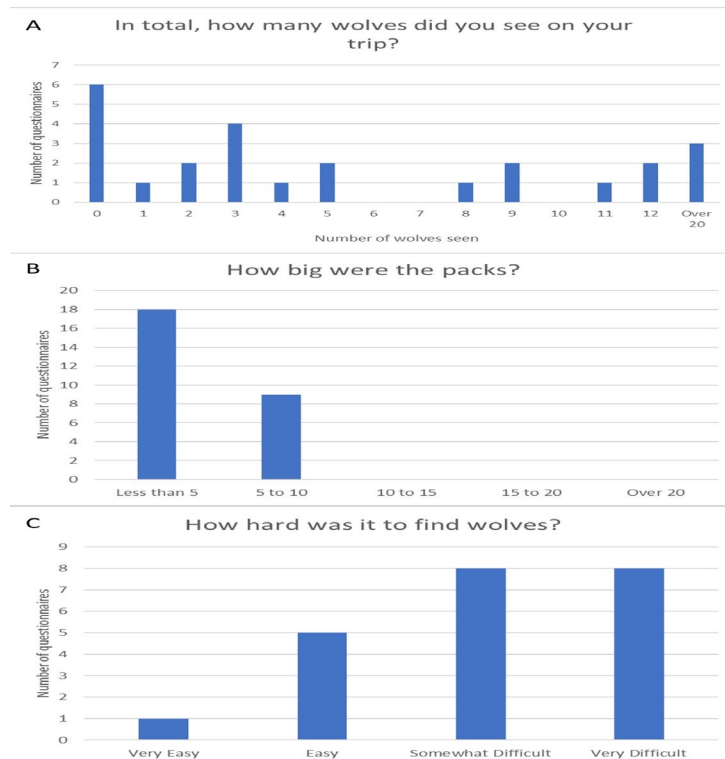
Figure 29. Qualitative summary of wolf sightings and effort reported in 2023 harvester questionnaires.
