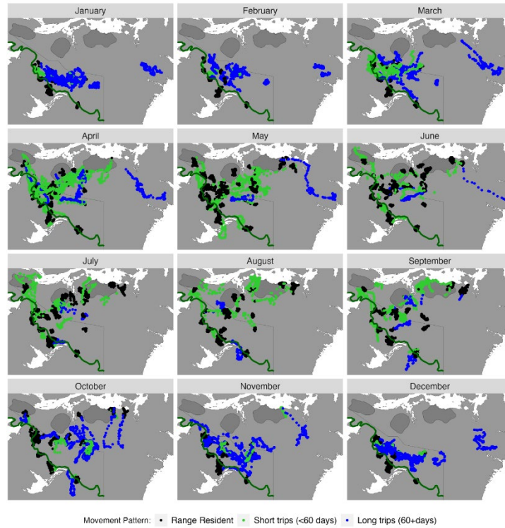
Figure 7. All movement patterns (range resident and non-range resident) of telemetry monitored tundra grey wolves (n=25) by month, March 2020 - March 2023. Datasets of wolves assigned to the range resident with short trips or range resident with short and long trips movement categories. Datasets pooled across years, not all deployments last the full time series. Grey polygons from west to east show calving grounds of the Bluenose-East, Bathurst and Beverly caribou herds respectively.
