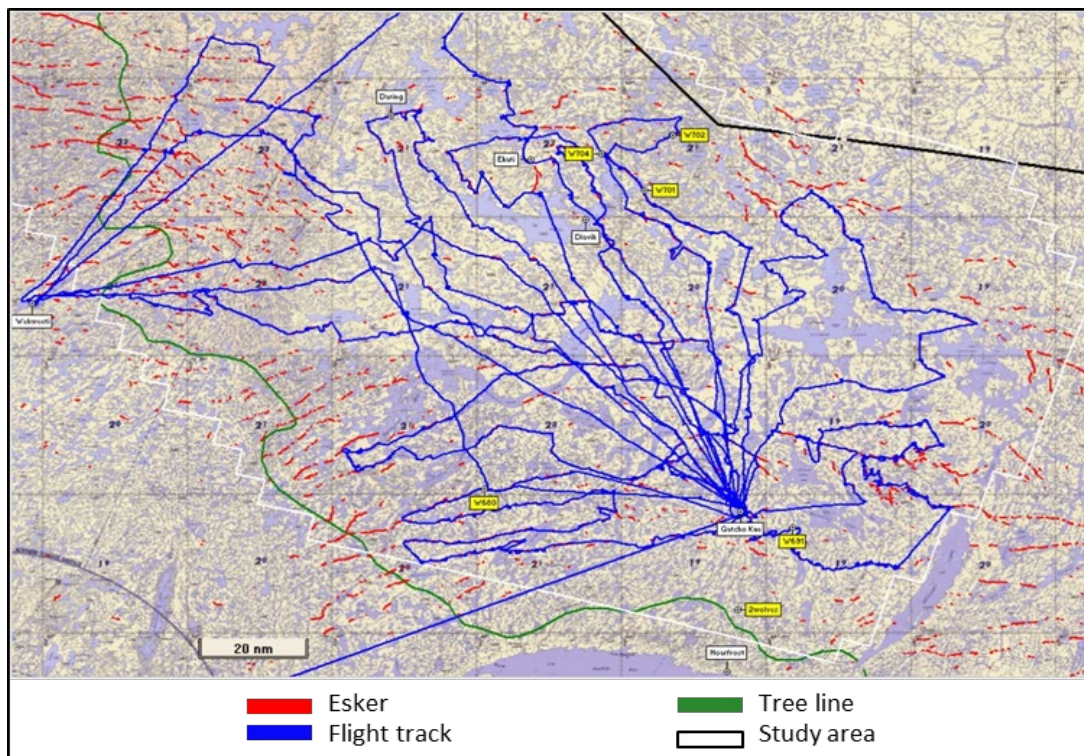
Figure 14. Study area and flight tracks for May 2023 wolf den survey. Yellow labels indicate wolf observations and white labels indicate places of interest.
