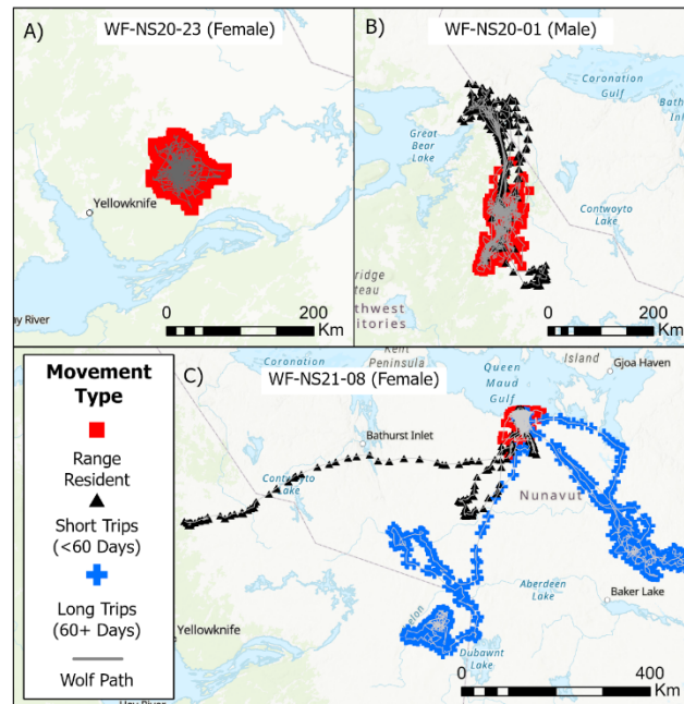
Figure 5. Representative maps of the three main movement patterns. A) exclusively range resident, B) range resident with short trips, C) range resident with short and long trips.
