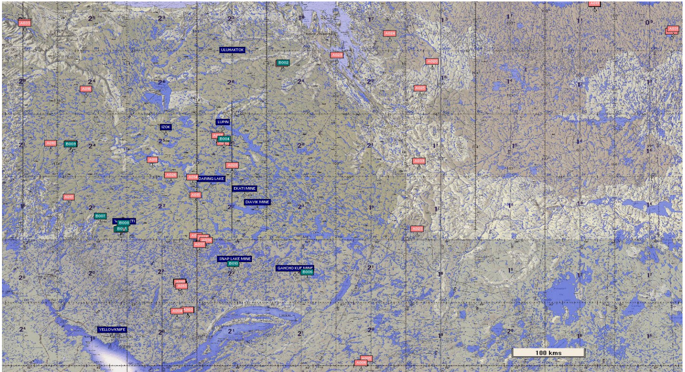
Figure 15. Wolf den sites identified using manual stratification of collar data from 2020 - March 2023 (AXX in pink) and the cluster algorithm of collar data from May-June 2023 (BXX in green). Only the locations using SR = 200 m, WD = 5 days, CML = ten locations are shown for the cluster algorithm dens. Places of interest are shown in blue.
