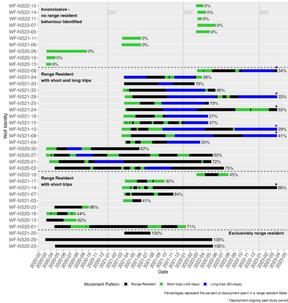
Figure 6. Movement patterns of telemetry monitored grey wolves.
