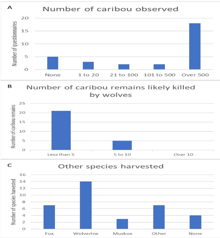
Figure 30. Qualitative summary of number of caribou observed and other harvests reported in 2023 harvester questionnaires.
