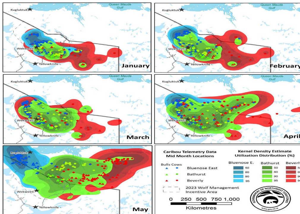
Figure 18. Monthly utilization distributions from January - May 2023 for Bathurst, Bluenose-East and Beverly caribou herds based on KDE.
