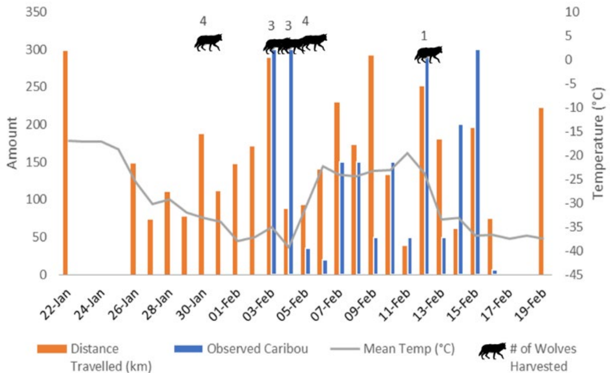
Figure 26. Data collected during the Tłıchǫ Government’s dıga harvesting camp in 2023 (Year 4); this includes the number of dıga harvested, number of ekwò seen, daily distance (km) travelled by hunters and mean daily temperature.
