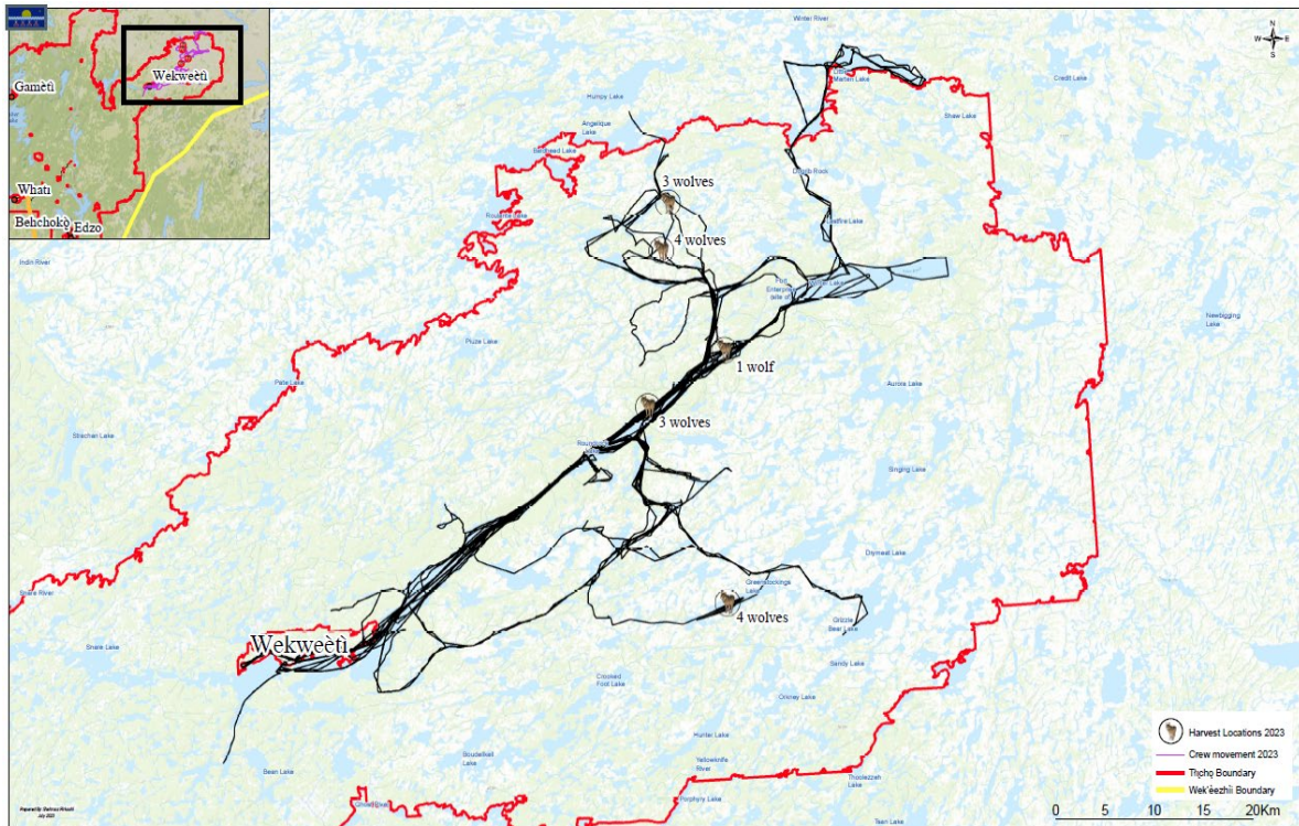
Figure 25. Snowmachine tracks (total of 3,778 km) and five kill locations for 15 harvested wolves during the fourth year (January - February 2023) of the Dìga Harvesting Program.
